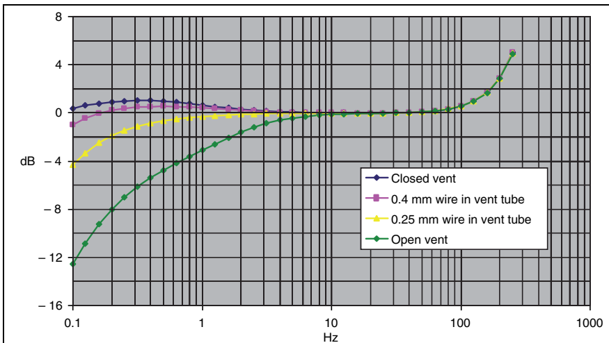
Fig. A1. Frequency response of active coupler as a function of venting conditions
